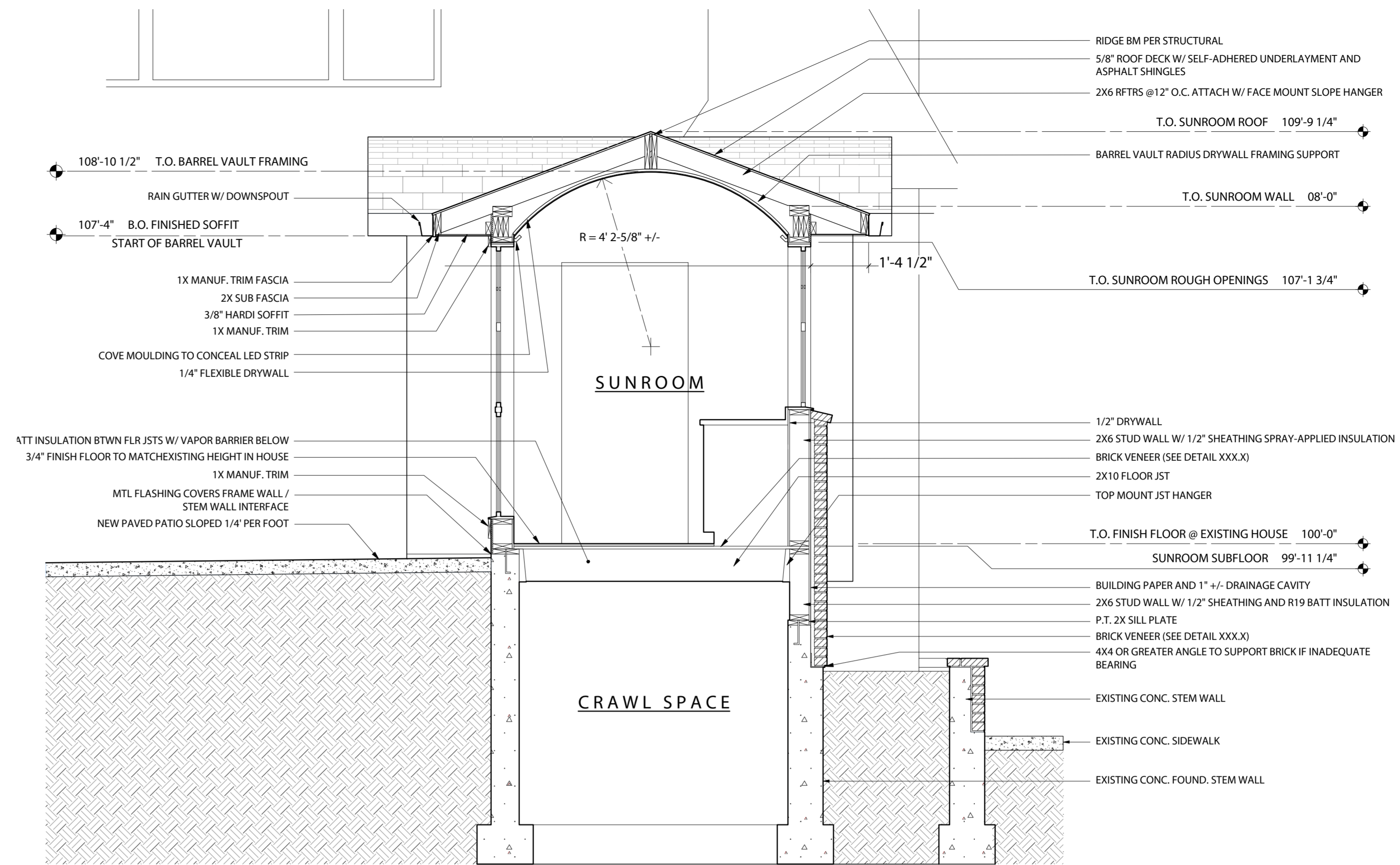
Sun Room Section Looking West
