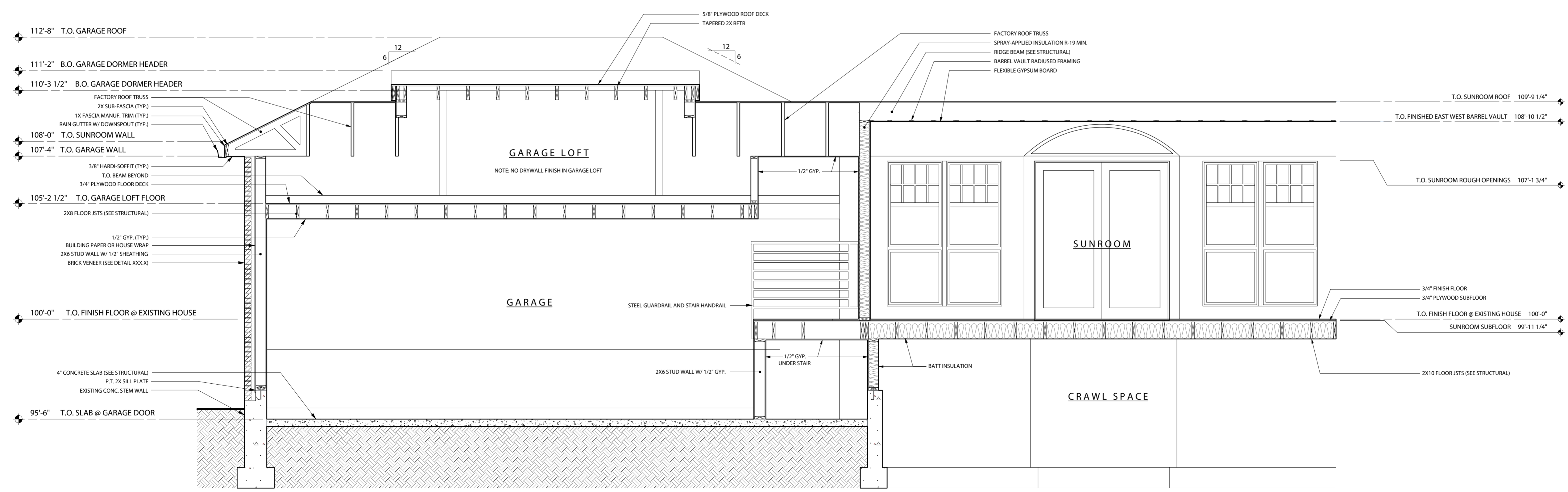
East West Longitudinal Section
