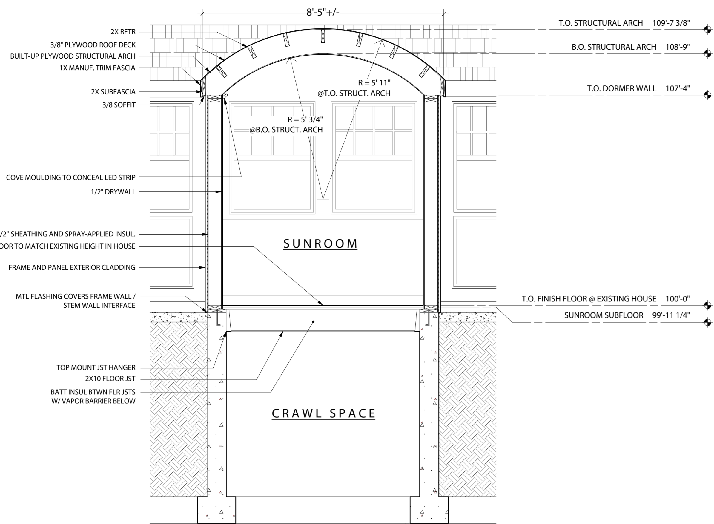
Sun Room Section Looking North
